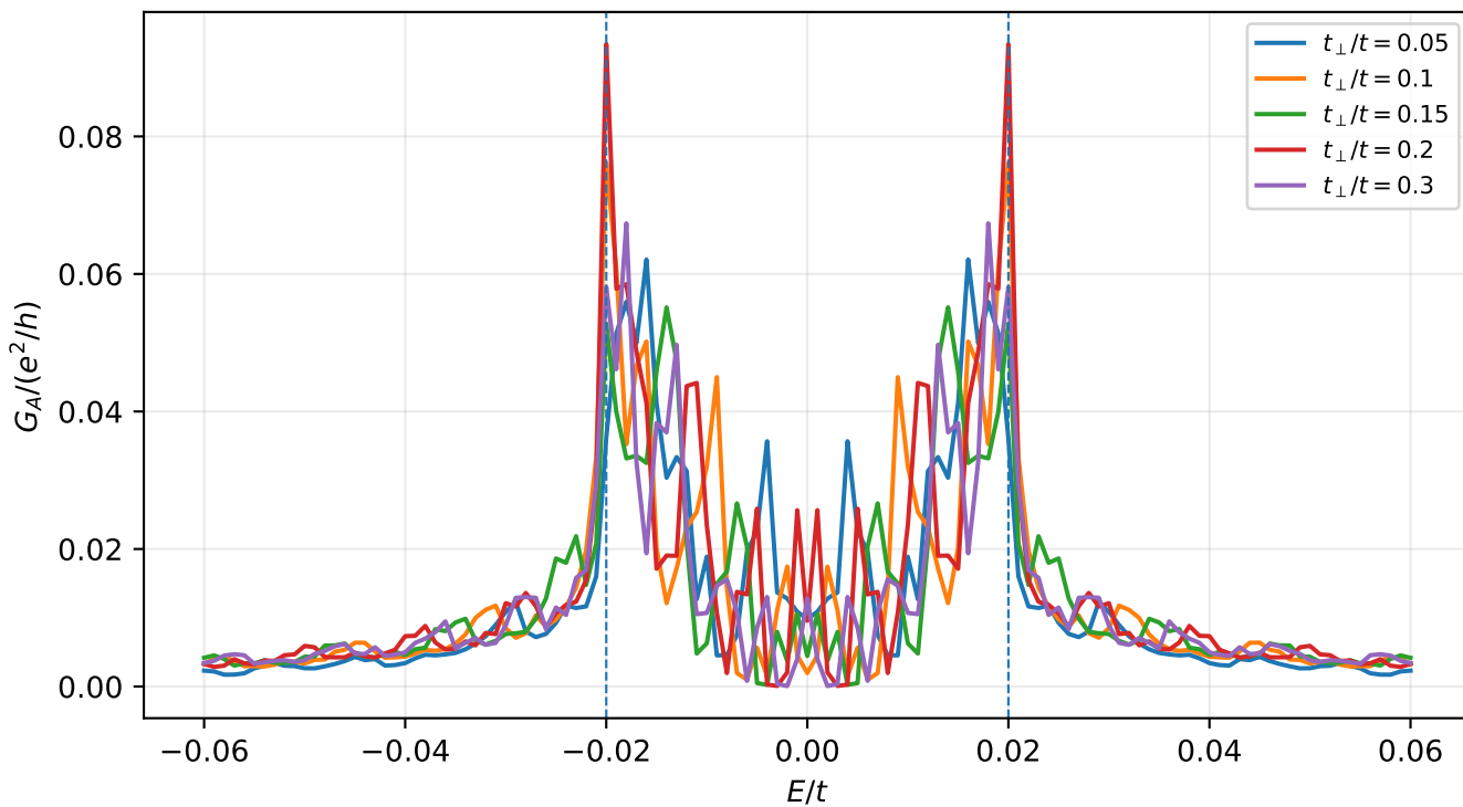
Interlayer coupling: G_A , 1to2
