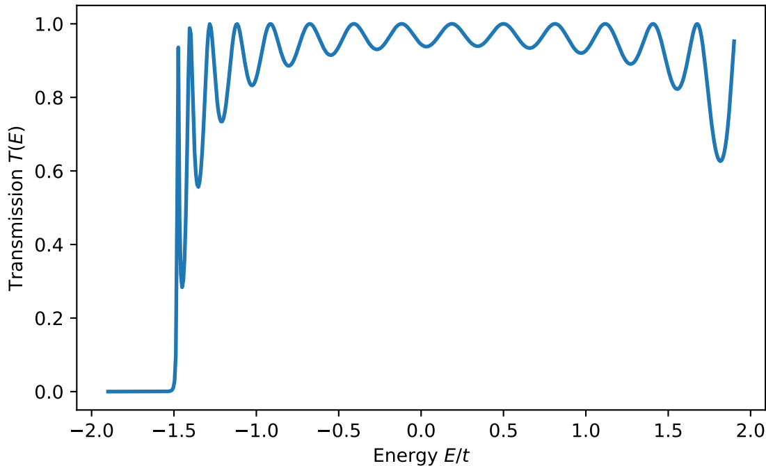
Transmission through a finite 1D barrier
