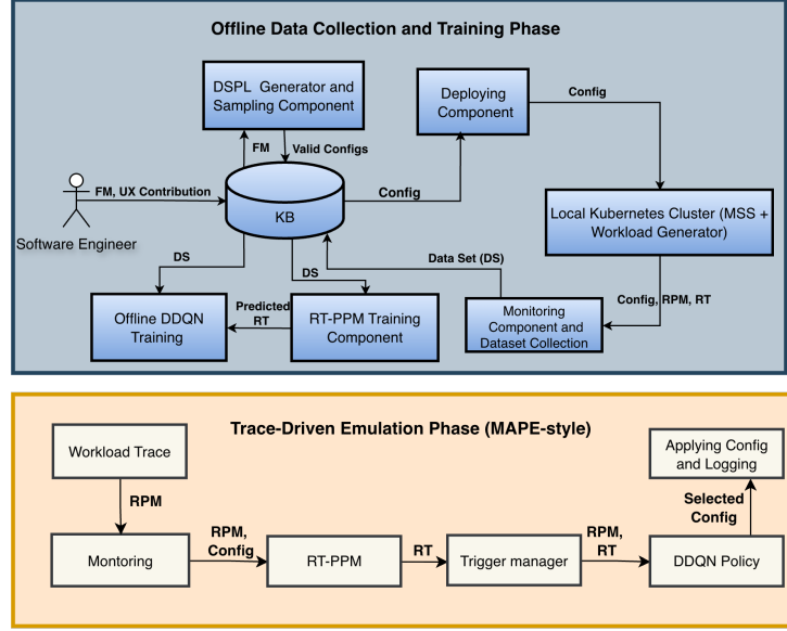
Fig. 2: Operational Framework of the DSPL-DRL Approach.
