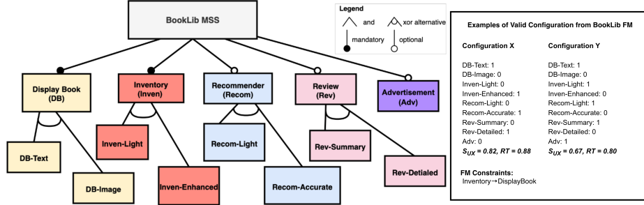
Fig. 1: Feature Model (FM) of the BookLib MSS with example valid configurations X and Y
