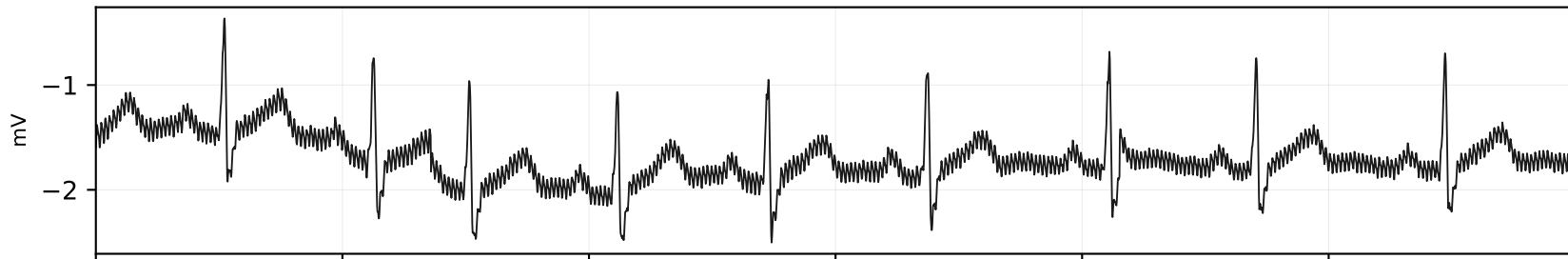
Sinal CRU — DIAG_MODE 1 (LeadII)
