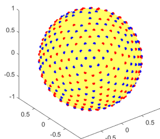
Figure 1: Q-ball
