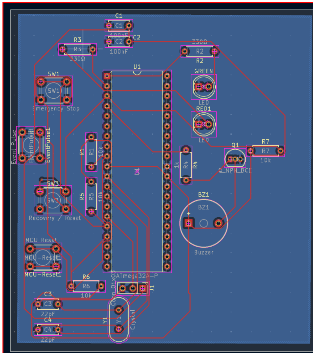
Figure 4: Final KiCad PCB layout.
