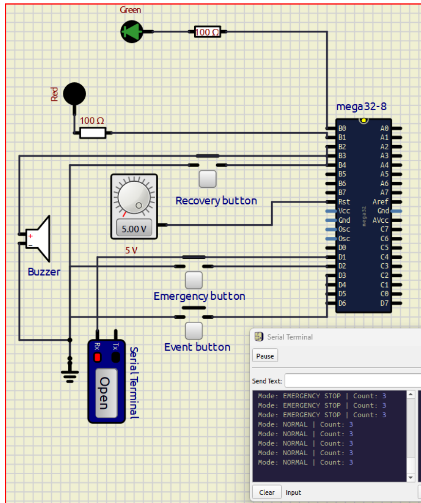
Figure 12: Recovery mode - system returns to normal mode.
