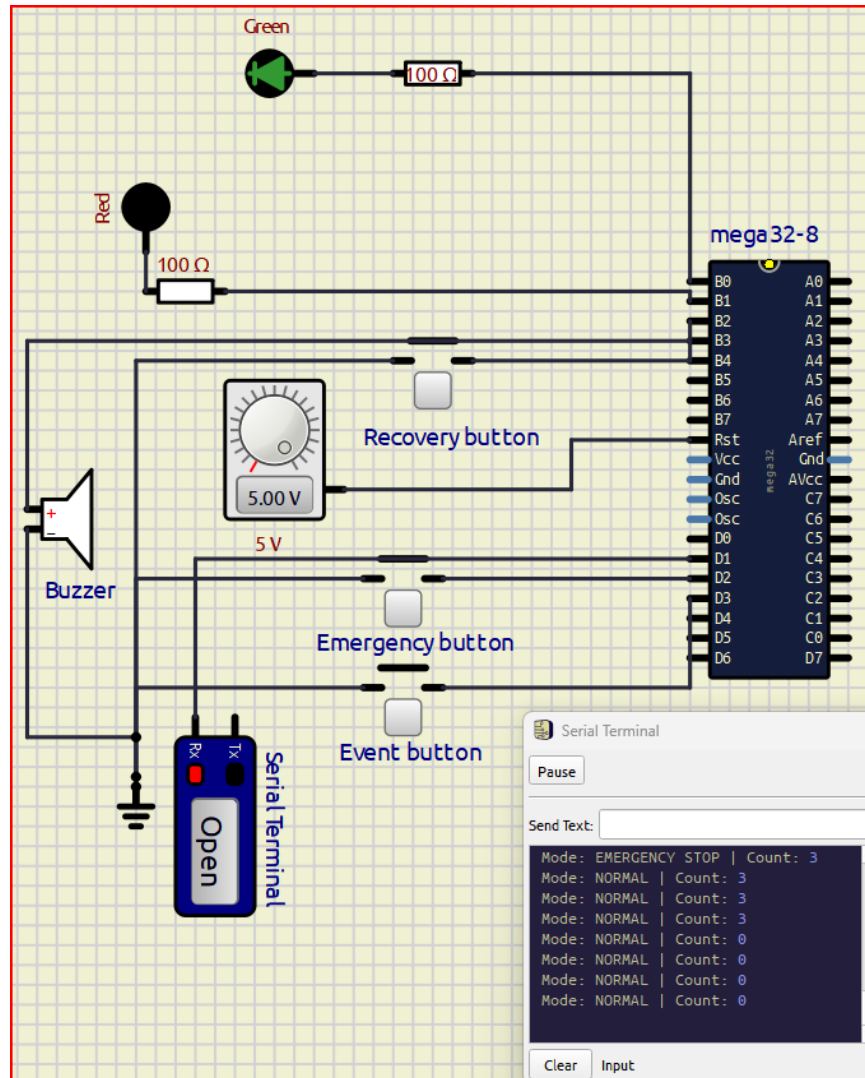
Figure 13: Reset in normal mode - count resets to 0.
