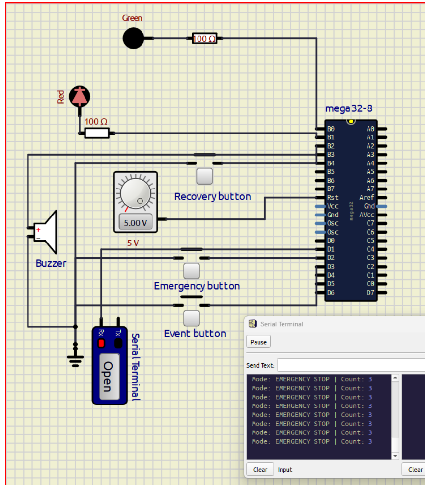
Figure 10: Emergency stop - emergency mode active.
