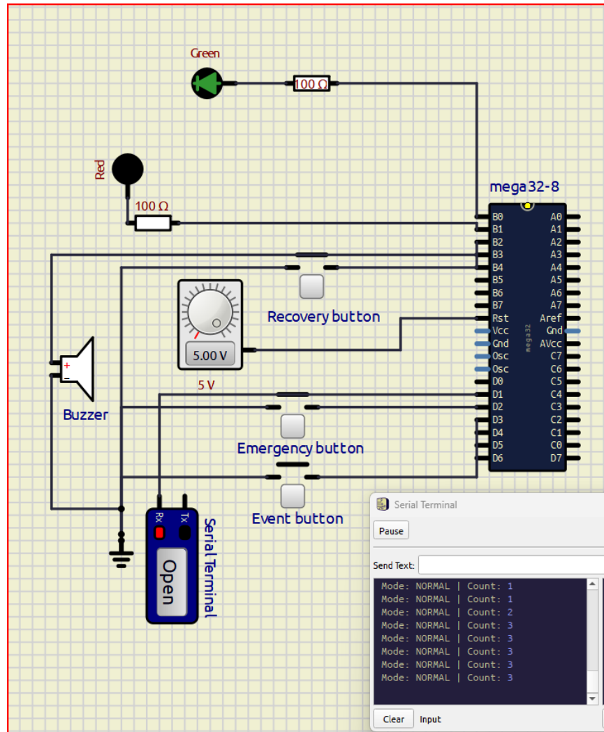
Figure 9: Multiple event pulses - count increases correctly.
