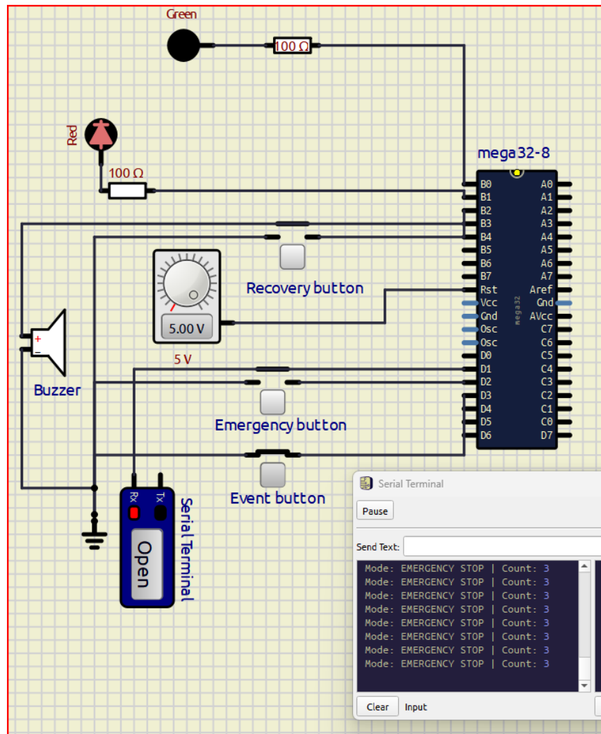
Figure 11: Event during emergency - count remains locked.
