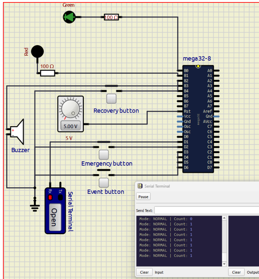
Figure 8: Single event pulse - count increases to 1.
