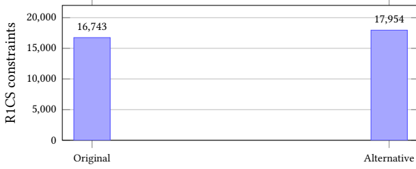
Figure 1: Local Circom size comparison: 16,743 versus 17,954 constraints, an increase of 1,211 (7.23%). The alternative changes the relation; this is not runtime overhead.
