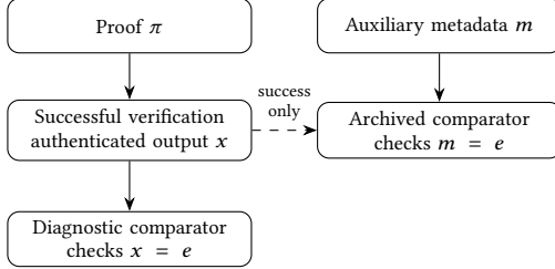
Figure 2: VeriSBOM’s tested data flow. The archived path gates on proof success but compares auxiliary values; the diagnostic path compares authenticated outputs. Arrows denote dependencies, not a measured causal model.
