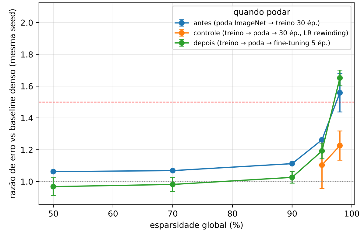
DenseNet-121
