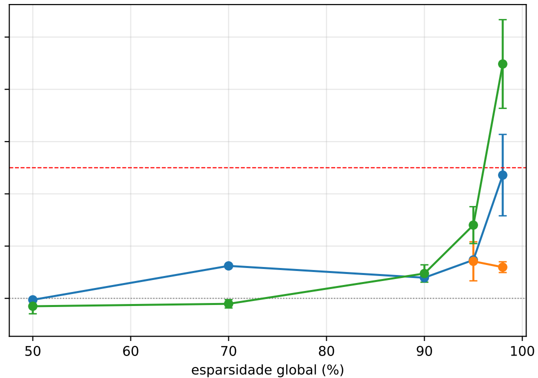
ResNet-50
