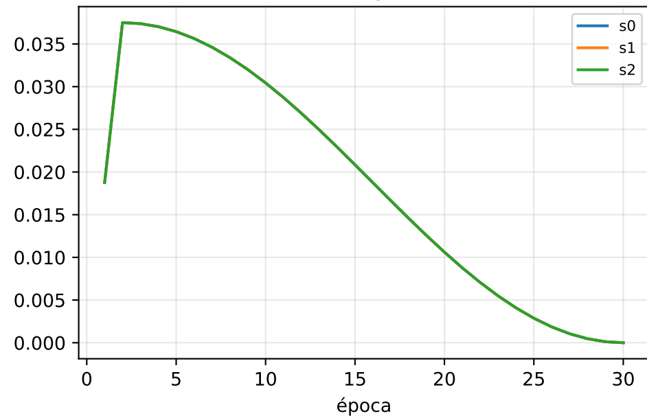
Learning rate
