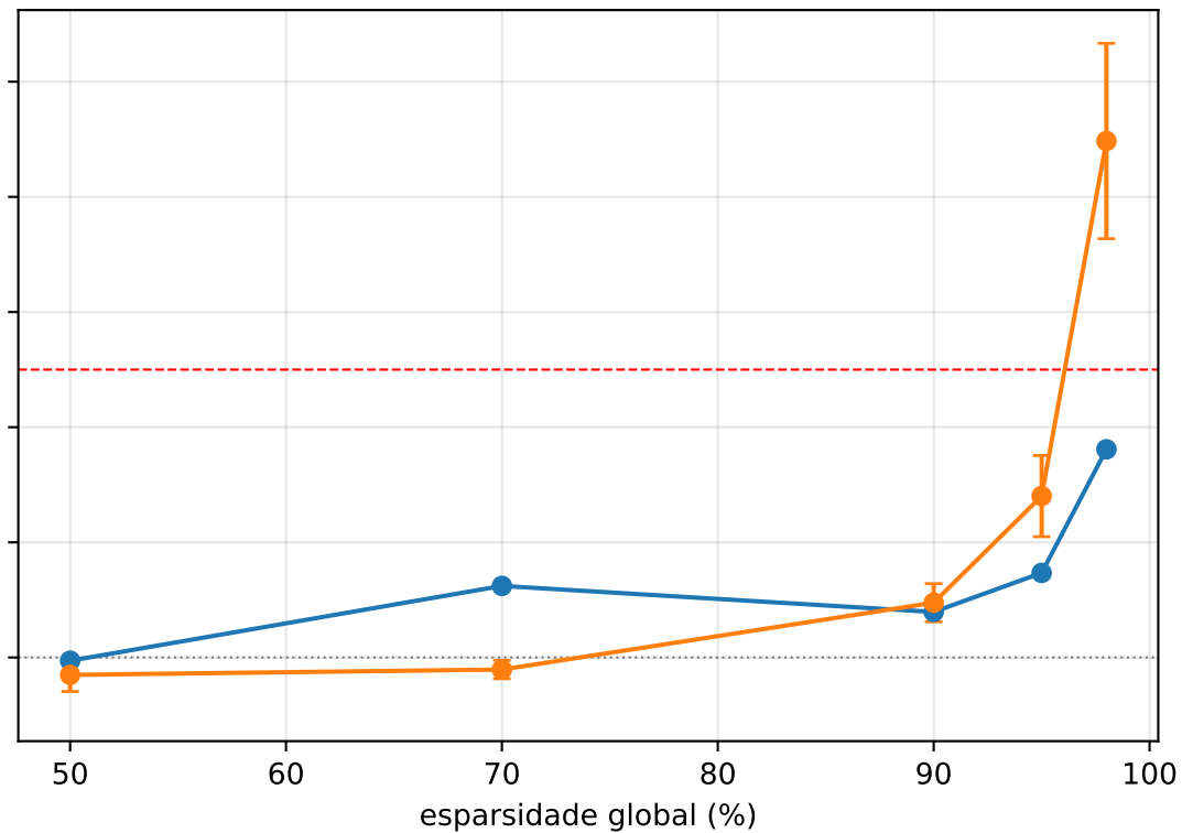
ResNet-50
