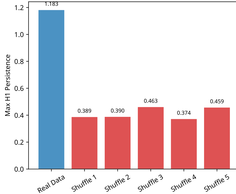
B. Real vs. Shuffled Spike Data (166 neurons)
