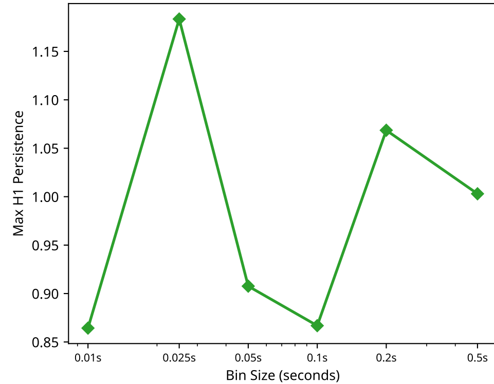
C. Effect of Temporal Resolution on Topology
