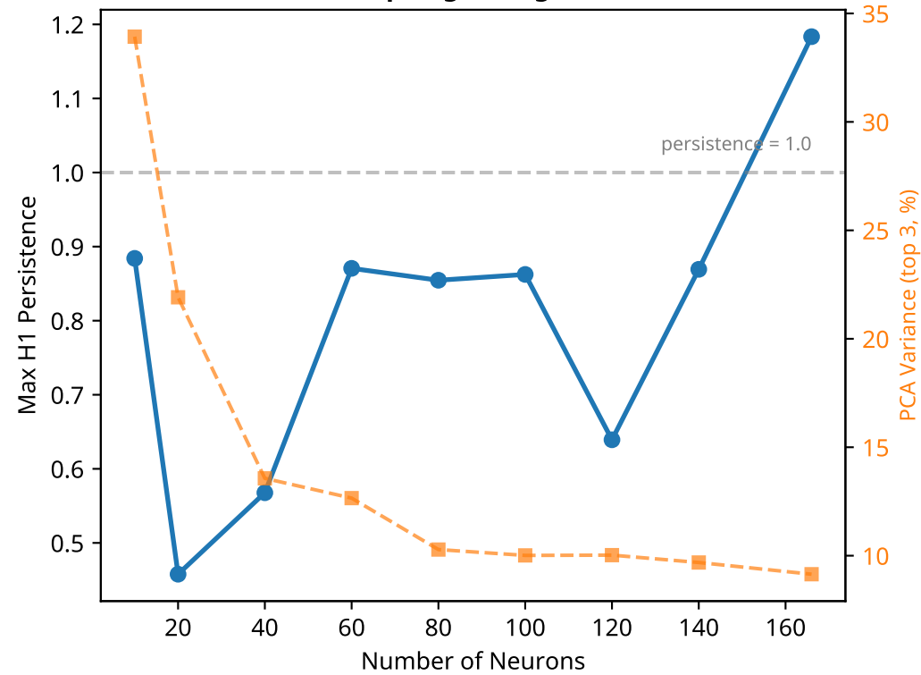
A. Effect of Population Size on Topological Signal
