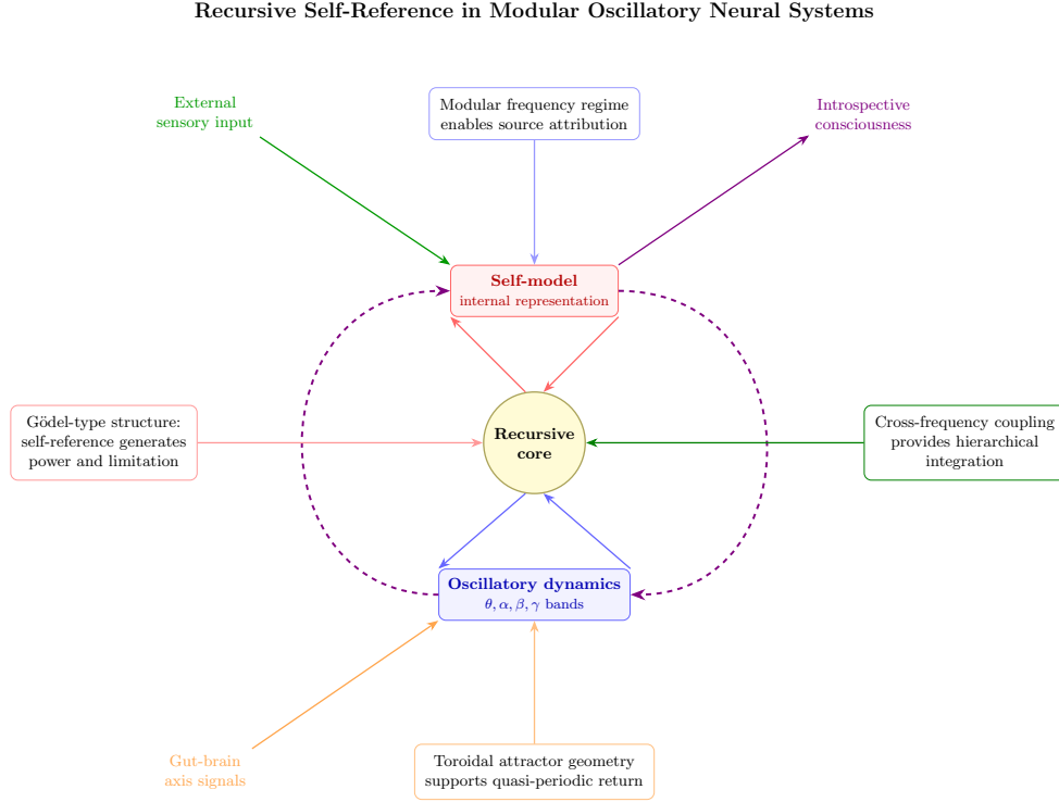
Figure 4: Recursive self-reference in modular oscillatory neural systems. The system generates representations of its own oscillatory states (inner loop), which are themselves subject to the same oscillatory dynamics (outer loop). This recursive structure, enabled by modular frequency organization and cross-frequency coupling, provides the computational basis for introspective consciousness. The toroidal attractor geometry supports quasi-periodic trajectories that continuously revisit previous states without exact repetition, creating a physical analogue of Gödel-type self-referential structure.
