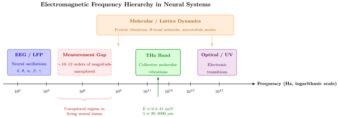
Figure 3: Electromagnetic frequency hierarchy in neural systems. The measurement gap between conventional electrophysiology (Hz to kHz) and molecular vibrational dynamics ( 10^9 to 10^{13} Hz) spans approximately 10 to 12 orders of magnitude. The terahertz band corresponds to collective molecular vibrations with photon energies matching thermal fluctuations and weak intermolecular forces in biological tissue.
