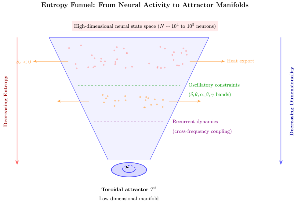
Figure 3: The entropy funnel: high-dimensional neural activity is progressively constrained by recurrent dynamics and oscillatory coupling onto low-dimensional attractor manifolds. The toroidal attractor T^2 represents a thermodynamically efficient geometry for encoding periodic information in phase relationships. Entropy decreases along the funnel axis as the effective dimensionality of the neural state is reduced.
