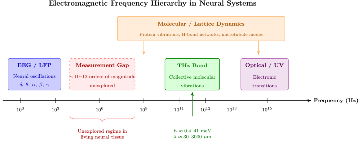
Figure 1: Electromagnetic frequency hierarchy in neural systems. The measurement gap between conventional electrophysiology (Hz to kHz) and molecular vibrational dynamics ( 10^9 to 10^{13} Hz) spans approximately 10 to 12 orders of magnitude. The terahertz band corresponds to collective molecular vibrations with photon energies matching thermal fluctuations and weak intermolecular forces in biological tissue.
