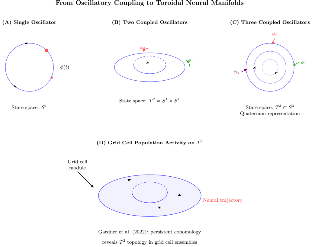
Figure 2: From oscillatory coupling to toroidal neural manifolds. (A) A single oscillator traces a circle S^1 . (B) Two coupled oscillators produce dynamics on the two-torus T^2 = S^1 \times S^1 . (C) Three coupled oscillators produce dynamics on T^3 \subset S^3 , naturally represented by unit quaternions. (D) Grid cell population activity from a single module resides on a toroidal manifold, as demonstrated by Gardner et al. [4] using persistent cohomology.
