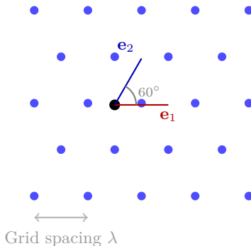
(C) Phase wrapping produces toroidal topology
