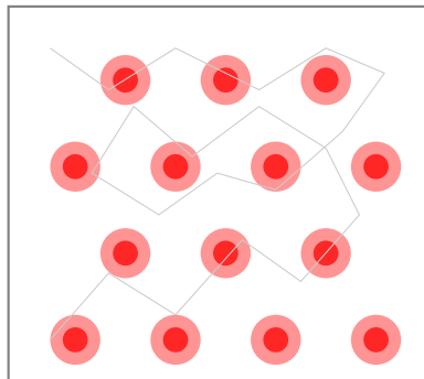
(A) Spatial firing fields
