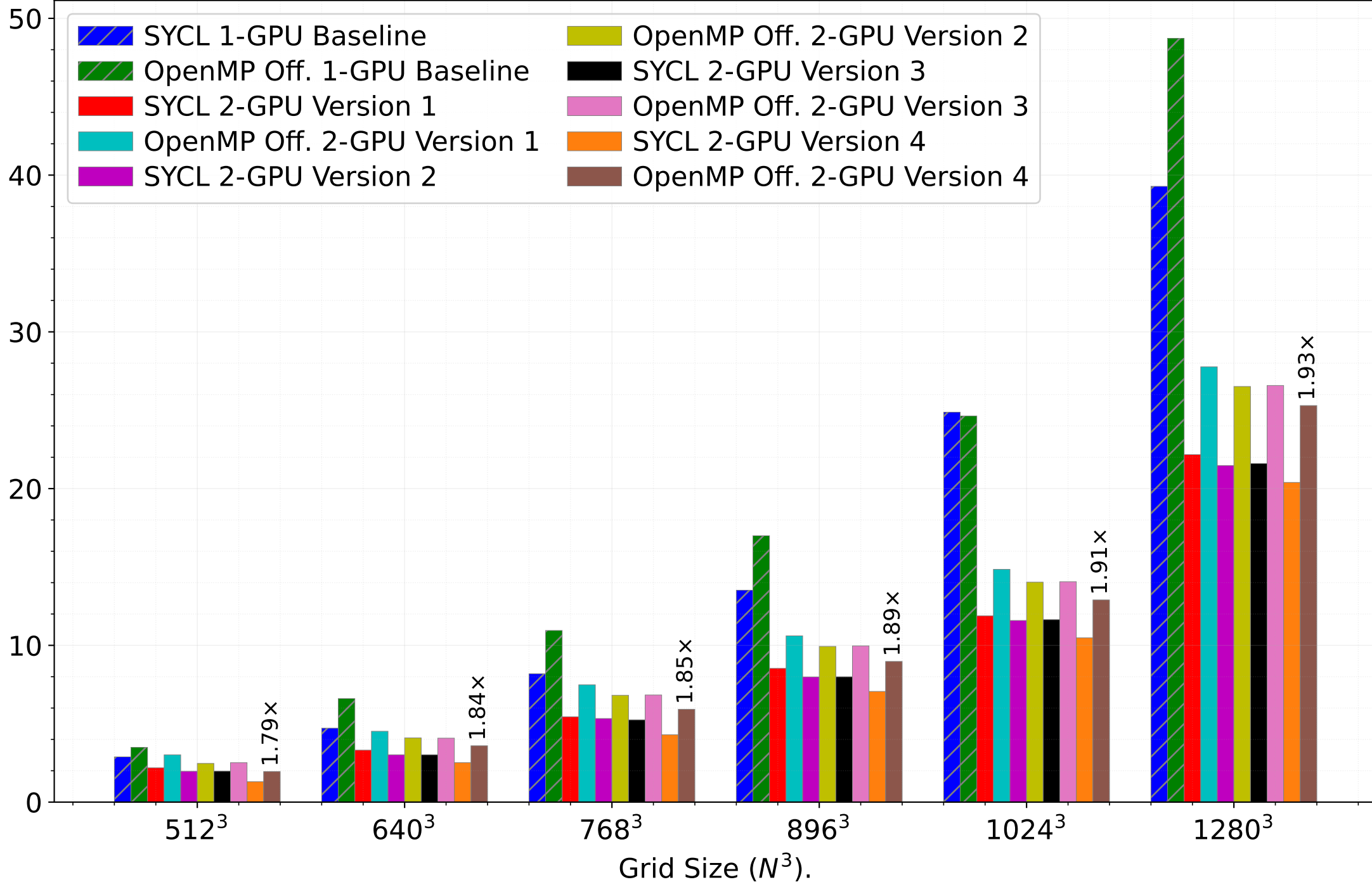
Intel Max 1550 - 2 GPUs (composite) (~500 time steps).
