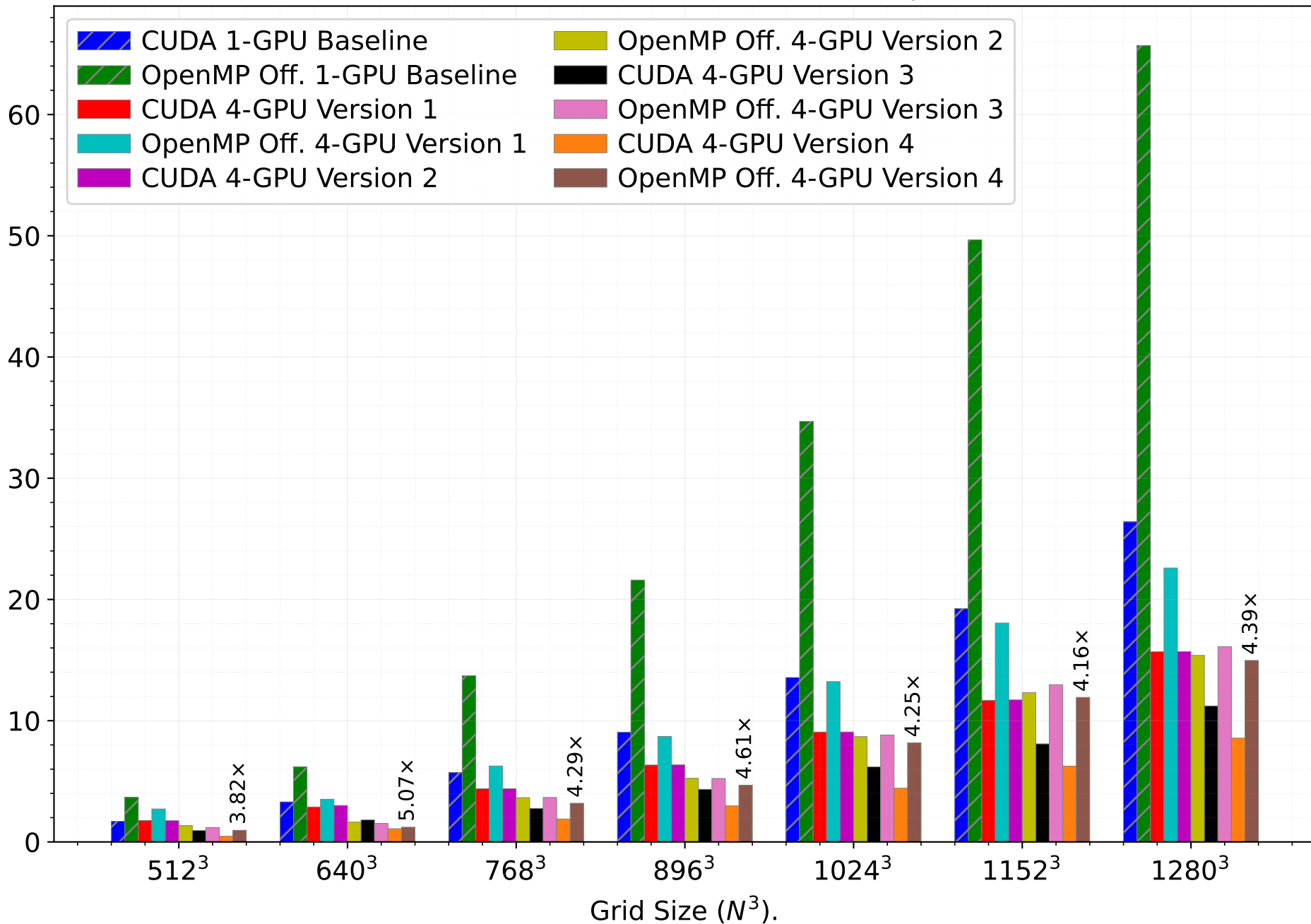
NVIDIA H100 - 4 GPUs (~500 time steps).
