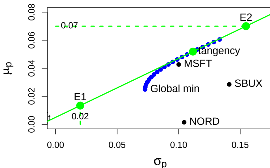
Figure 11.10: Tangency portfolio
