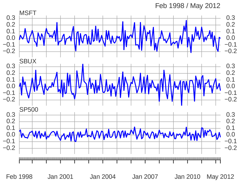
Figure 6.11: Simulated GWN model returns on Microsoft, Starbucks and the S&P 500 Index.
