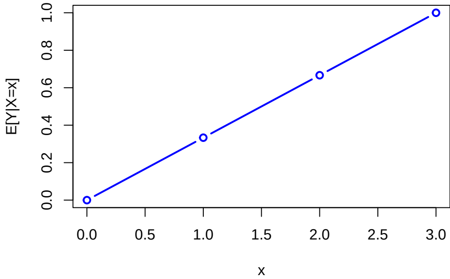
Figure 2.11: Regression function E[Y|X = x] from discrete bivariate distribution.
