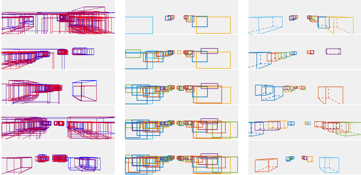
Figure 7: Qualitative examples of car detections results: (left) top 50 scoring proposals (color from blue to red indicates increasing score), (middle) 2D detections, (right) 3D detections.
