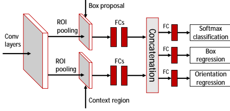
Figure 2: CNN architecture adopted from [10] used to score our proposals for object detection and orientation estimation.
