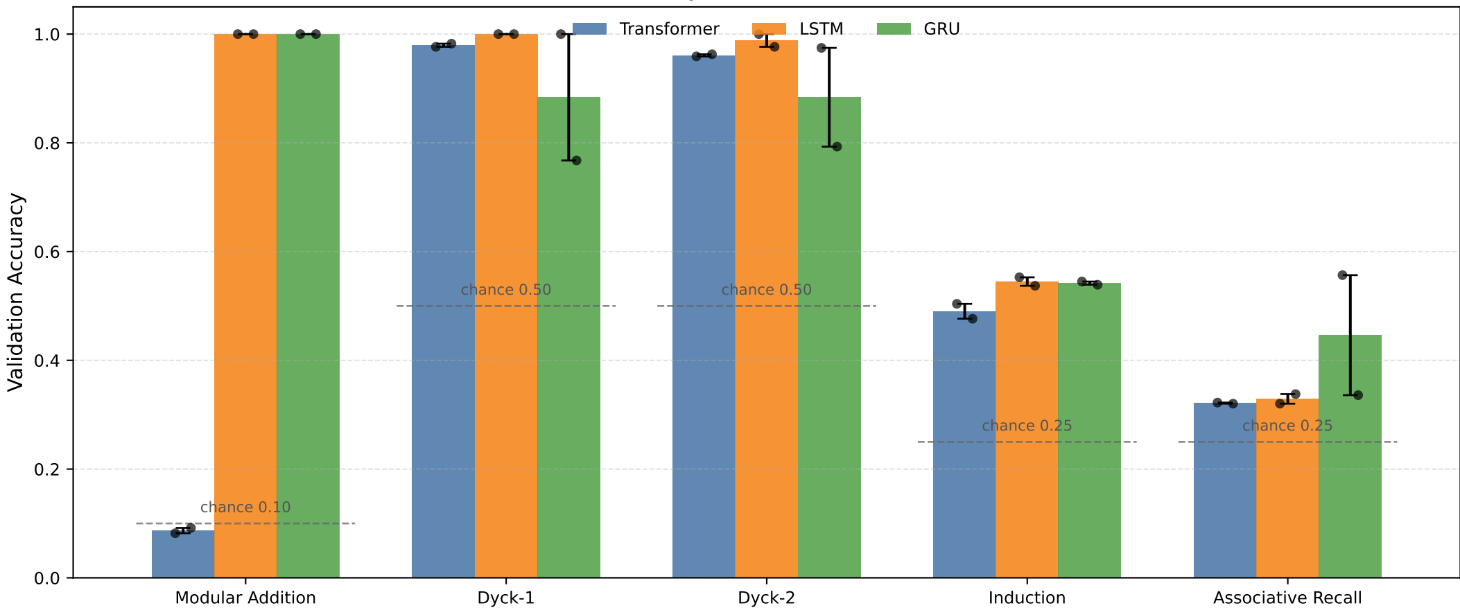
Validation Accuracy Across Tasks and Architectures
