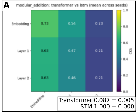
Modular Addition: Transformer vs LSTM
