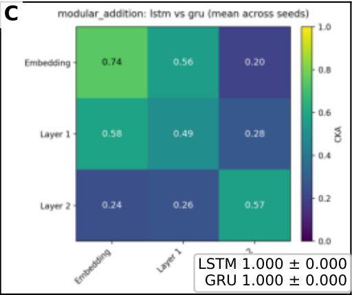
Modular Addition: LSTM vs GRU
