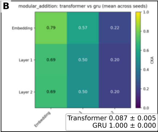
Modular Addition: Transformer vs GRU
