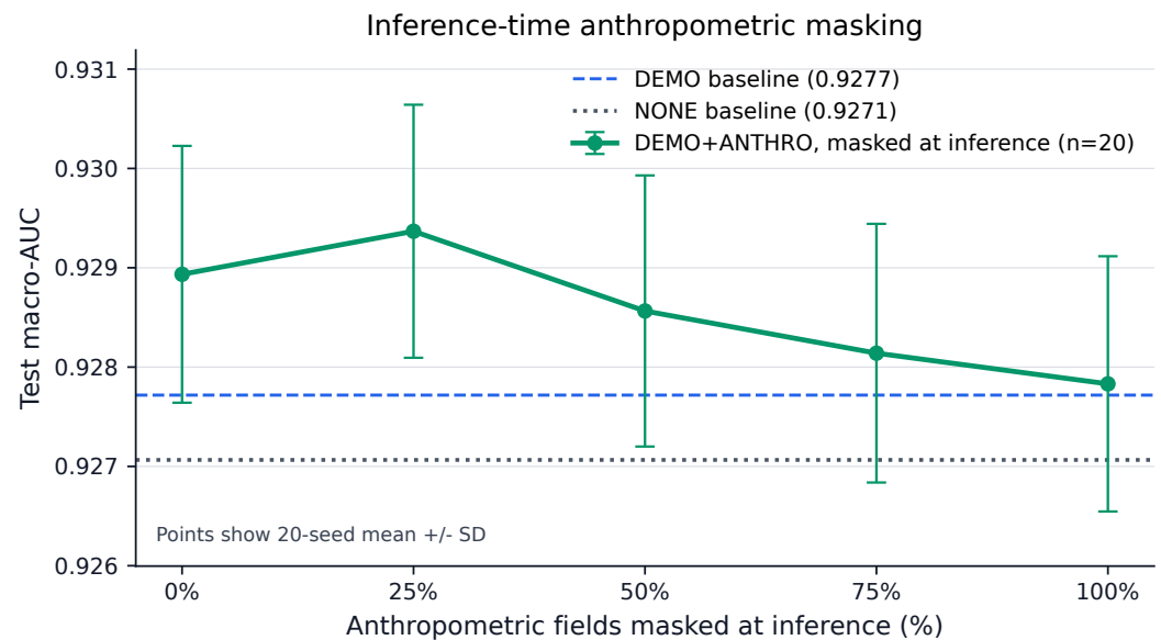
Figure 4. Missingness robustness of the availability-aware fusion pathway. The demo+anthro empirical masking curve is evaluated across 20 seeds (seeds 2024–2043); none and demo traces are structural reference baselines (immune to anthropometric masking by construction) shown at their 20-seed mean. Test macro-AUC is shown as a function of the fraction \rho of anthropometric fields withheld at inference (MCAR, independently per field); dashed horizontal lines show the demo and none baselines. Full masking ( \rho=1.0 ) costs \approx 0.0011 macro-AUC for demo+anthro, converging to the demo baseline (difference +0.00011 , within one-tenth of the cross-seed SD); the none variant is immune by construction. Availability-mask updating is performed consistently at each rate.
