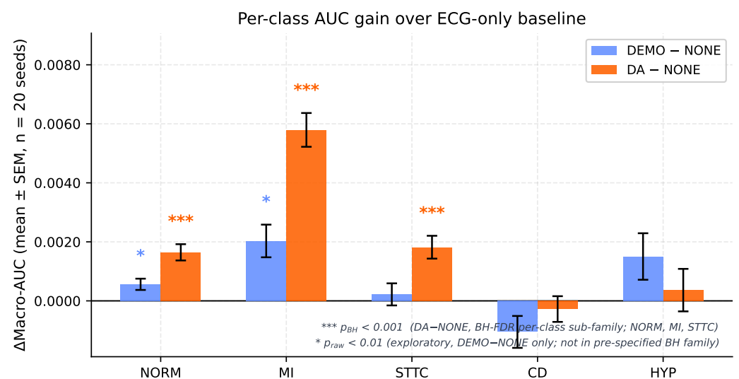
Figure 3. Per-class \Delta -AUC of demo and demo+anthro relative to none, mean \pm paired SEM across 20 seeds . Orange markers (DA – none): *** = p_{\text{BH}} < 0.001 (BH-FDR corrected within the per-class DA – NONE sub-family; all three significant classes NORM, MI, STTC reach p_{\text{BH}} < 0.001 ). Blue markers (DEMO – none): * = p_{\text{raw}} < 0.01 (exploratory, not in the pre-specified BH family; NORM p = 0.006 , MI p = 0.003 ). CD and HYP show no significant gain in either contrast.
