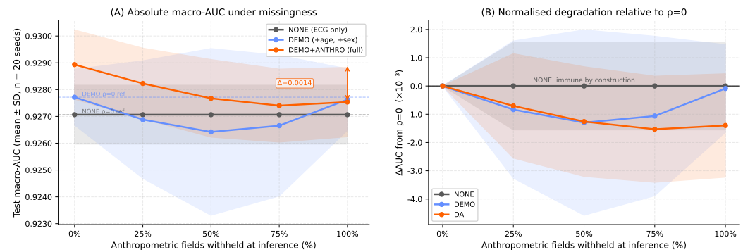
Figure 4. Missingness robustness of quality-gated fusion across 20 seeds. (A) Test macro-AUC as a function of the fraction \rho of anthropometric fields withheld at inference (MCAR); dashed horizontal lines show each variant's \rho=0 baseline; the double-headed arrow quantifies the degradation cost. (B) Normalised degradation \Delta AUC = AUC(\rho) - AUC(0) in units of 10^{-3} for direct cross-variant comparison. Full masking ( \rho=1.0 ) costs \approx 0.0014 macro-AUC for demo+anthro, converging to the demo baseline (difference -0.00018 , within \frac{1}{6} SD); the none variant is immune by construction. Availability-mask updating is performed consistently at each rate.
