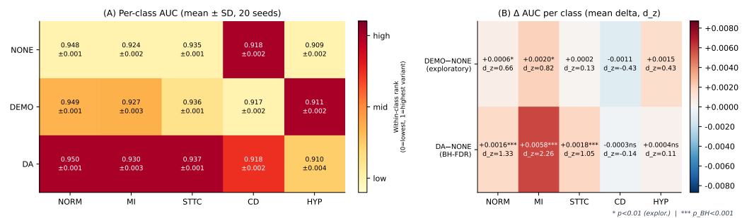
Figure 5. Per-class performance decomposition across 20 seeds. (A) Per-class AUC for the three ablation variants (mean \pm SD); colormap is normalised within each class column so that within-class variant differences are perceptually visible. (B) \Delta AUC delta matrix: top row = demo—none (exploratory, threshold p < 0.01 ); bottom row = demo+anthro—none (BH-FDR corrected within per-class sub-family). Each cell shows \Delta mean and Cohen's d_z . MI shows the largest absolute shift ( +0.0058 , d_z = 2.26 , p_{BH} < 0.0001 ). NORM and MI already reach significance under demographics alone (top row, p < 0.01 ); STTC additionally reaches significance only with full anthropometrics (bottom row, p_{BH} = 0.00035 ). CD and HYP show no significant gain in either contrast.
