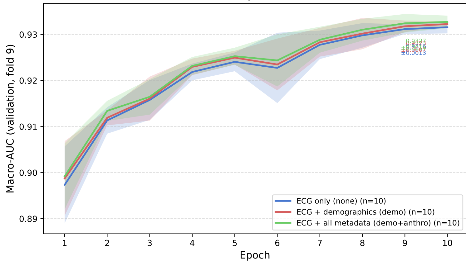
Validation AUC trajectory — mean \pm SD across 10 seeds (shaded region = \pm 1 SD)
