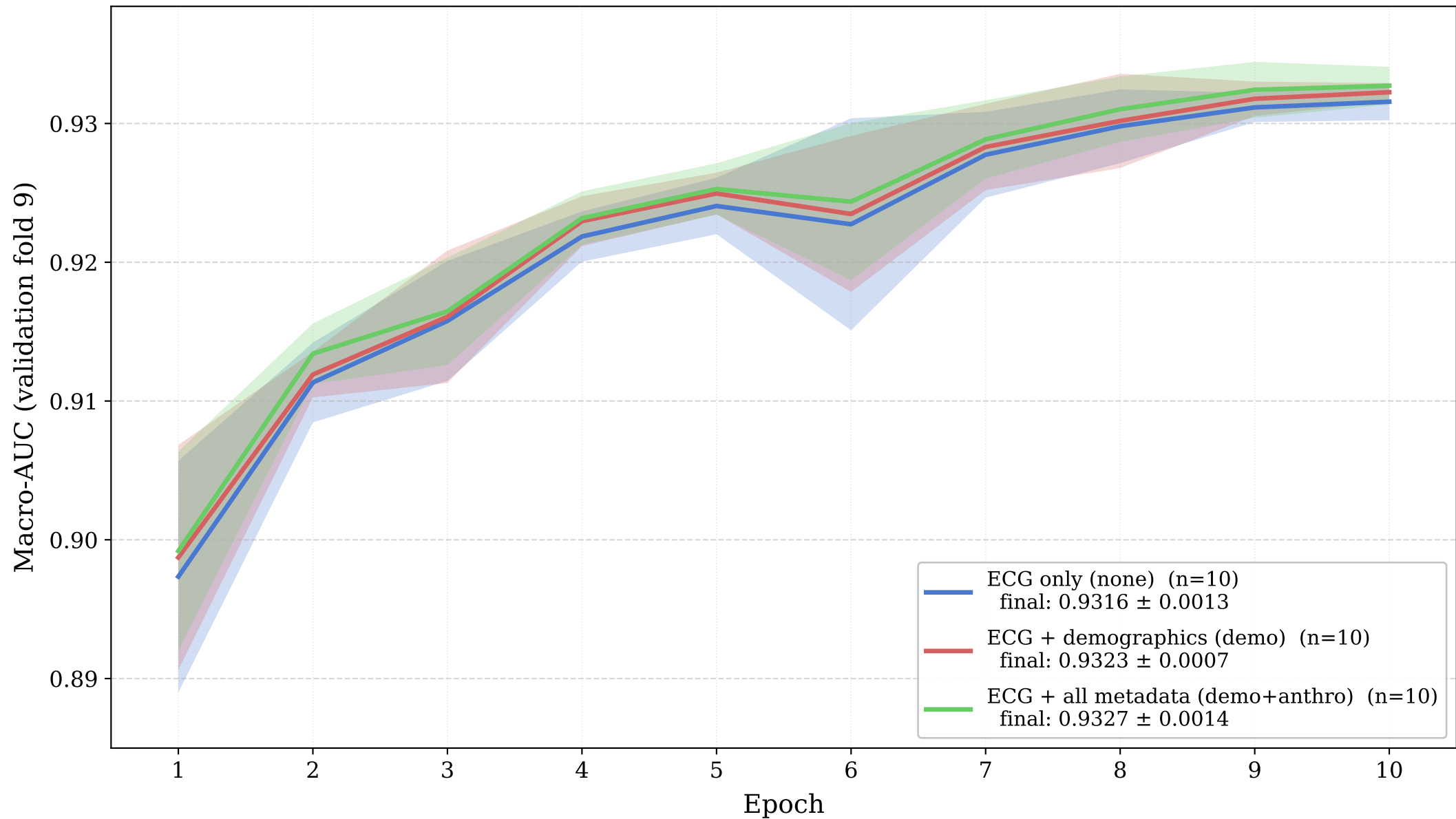
Validation macro-AUC trajectory — mean \pm 1 SD across 10 seeds
