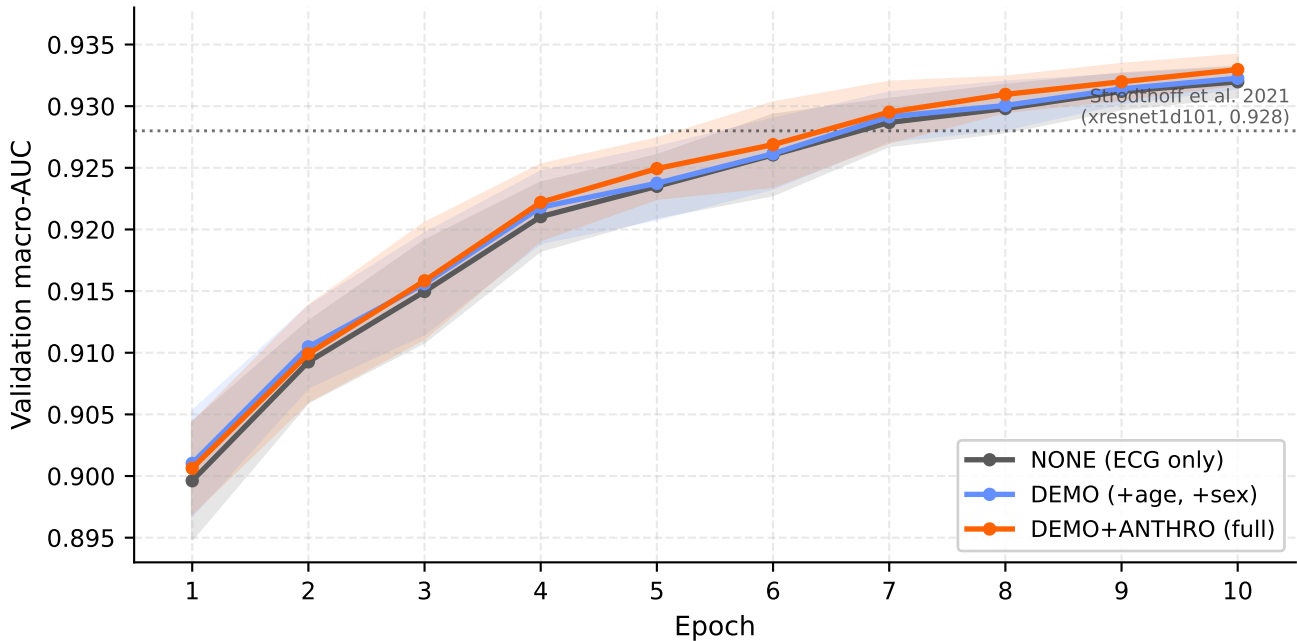
Training dynamics (mean \pm SD, n = 20 seeds, eval on fold 9)
