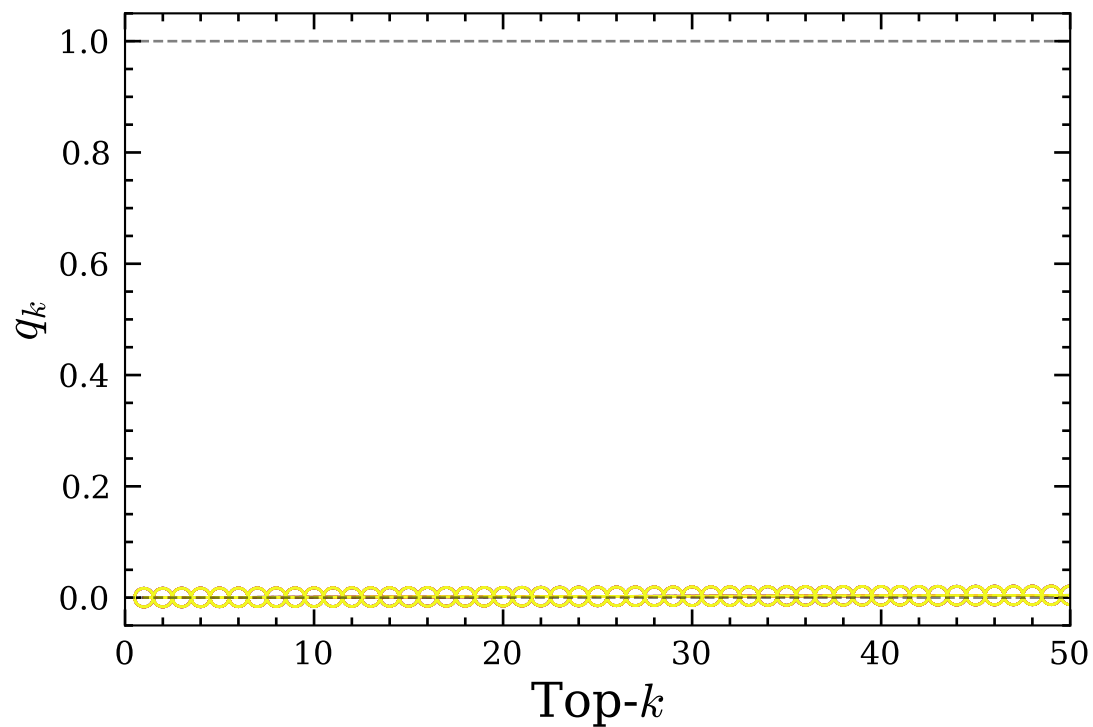
DISORDERED, \epsilon = 0.00000195 , 1/\sigma_W = 0.00195
