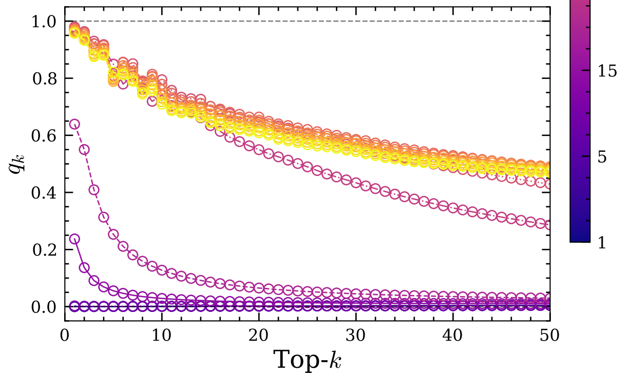
FERROMAGNETIC, \epsilon = 0.008 , 1/\sigma_W = 8
