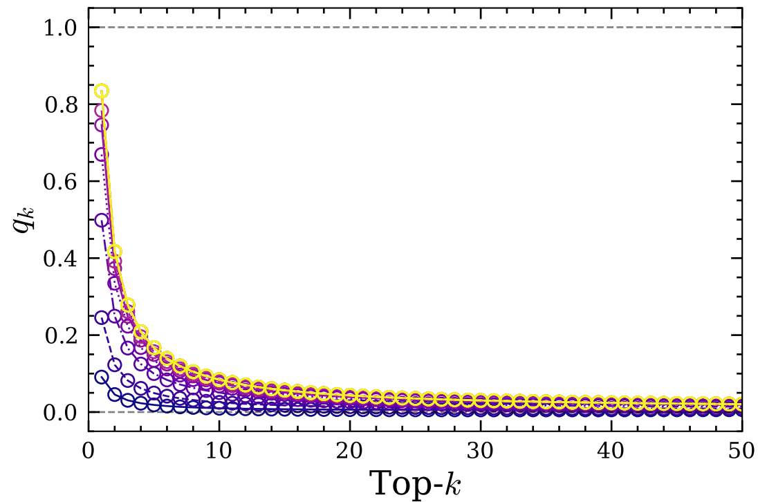
DISORDERED, \epsilon = 9.54 \times 10^{-7} , 1/\sigma_W = 1.96 \times 10^{-3}
