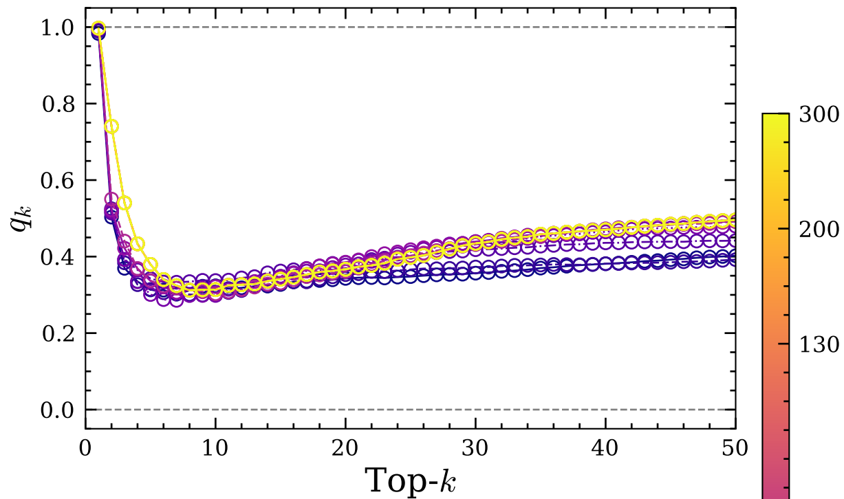
FERROMAGNETIC, \epsilon = 0.0039 , 1/\sigma_W = 8
