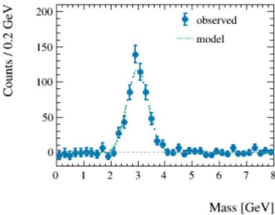
Background subtraction
