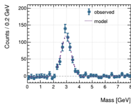
Background subtraction
