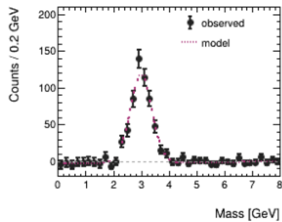
Background subtraction
