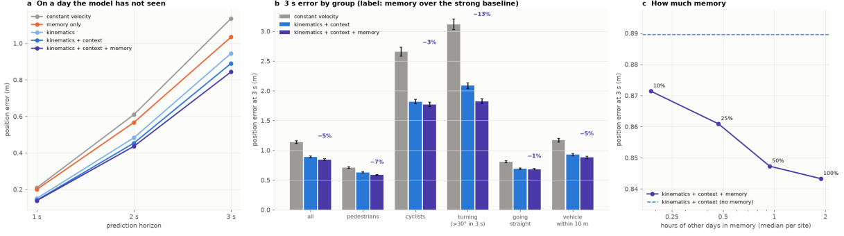
Figure 16: Forecasts of pedestrians and cyclists on a day the model has not seen (inD, leave-one-session-out). (a) Position error by horizon. (b) Error at 3 s by group, with 95 % intervals resampling whole tracks; labels give the change from adding memory to the strong baseline (kinematics + context). (c) Error with memory built from a fraction of the other days’ recordings.
