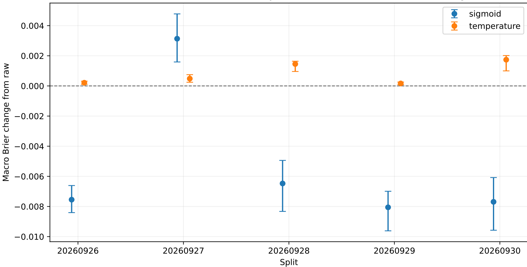
Deleting one evaluation artist at a time Whiskers are min/max sensitivity, NOT confidence intervals; no refitting
