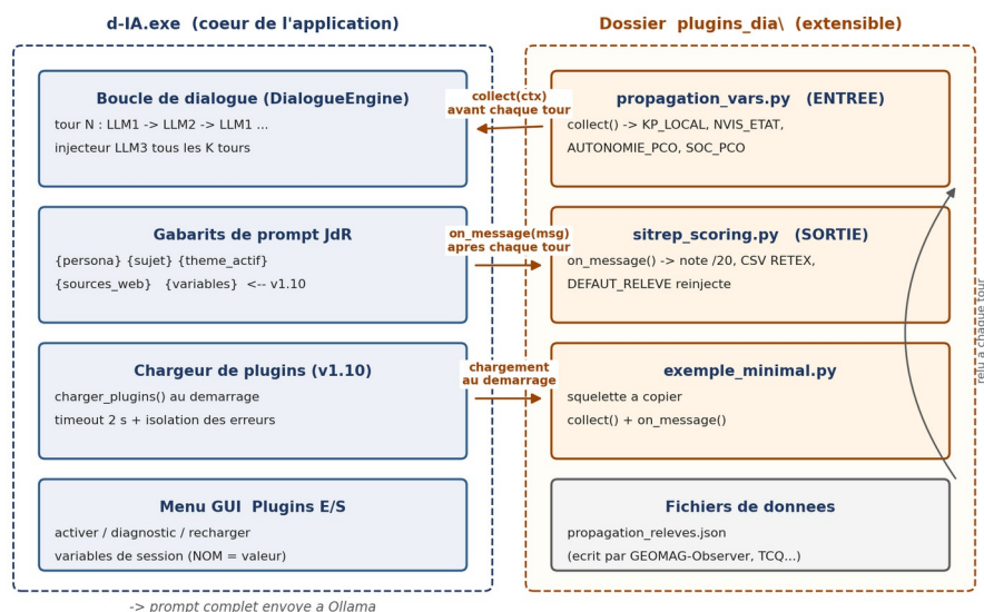
Figure 1 — Architecture du système de plugins d-IA v1.10
