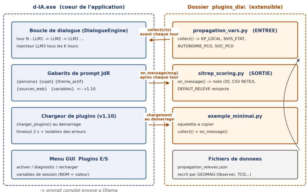
Figure 1 — Architecture du système de plugins d-IA v1.10
