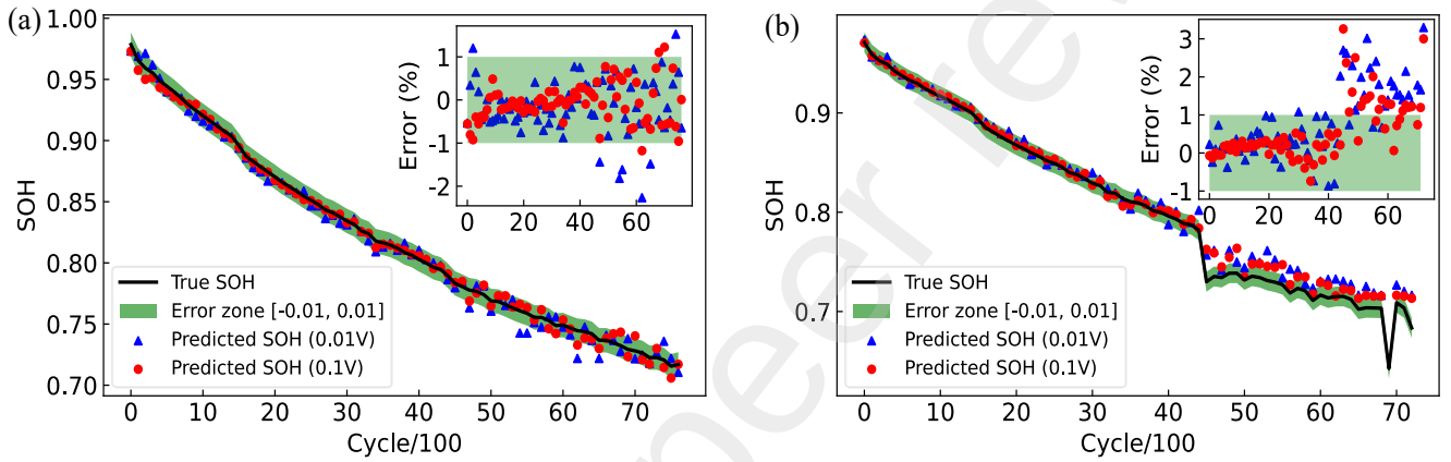
Fig. 5. SOH estimation results based on Random Forest regression. Oxford dataset (a) cell 1# and (b) cell 2#.
