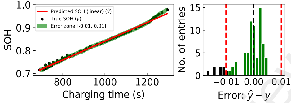
Fig. 4. Linear regression fitting and error diagram of 3.77 V to 3.87 V charging process of Oxford cell 1#.
