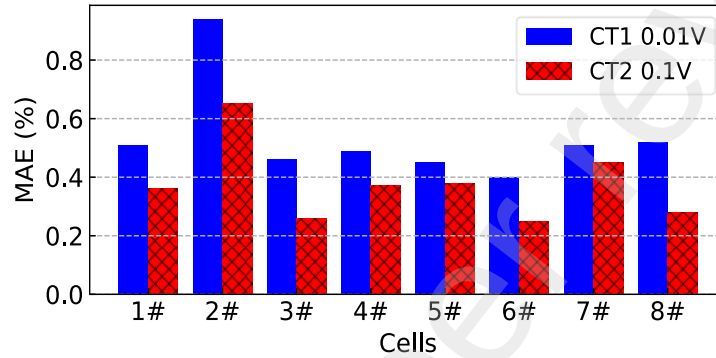
Fig. 6. MAE comparison chart of CT1 and CT2 estimation methods.
