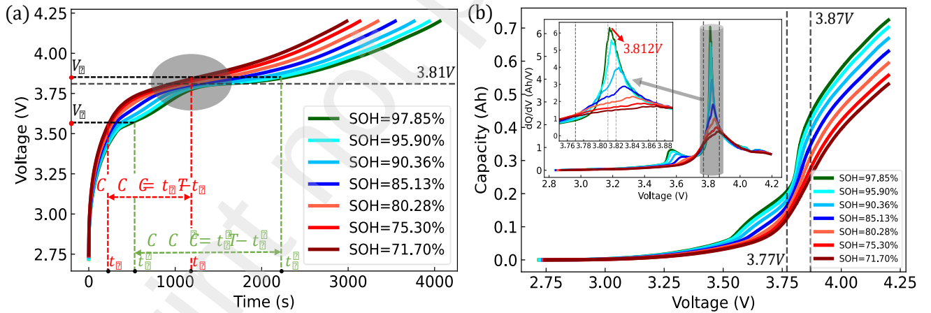
Fig. 2. Battery capacity degradation analysis (Oxford dataset cell 1#). (a) Charging voltage curves at different aging stages. (b) Capacity voltage curve and incremental capacity curve.
