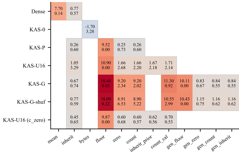
regret at sites (top) and leak \times 10^{-3} bpb (bottom)
