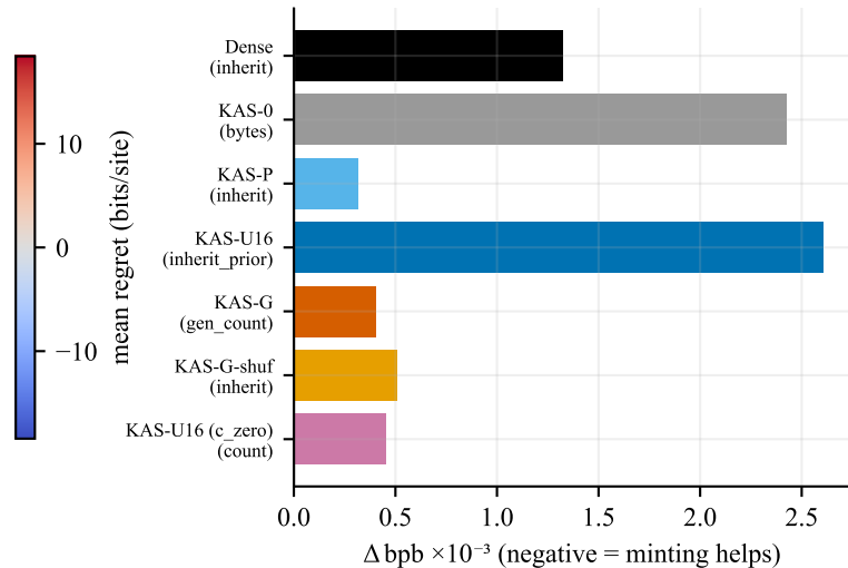
net effect on re-tokenised text
