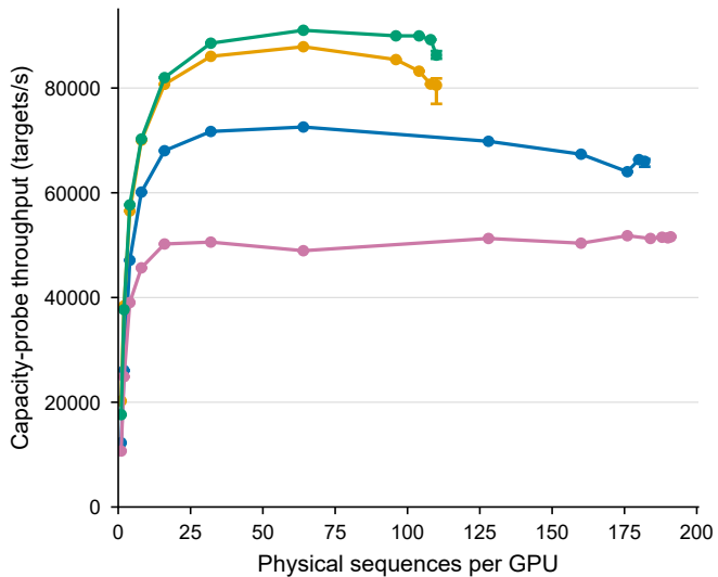
20-update capacity probes; concurrent workers; not isolated benchmarks
