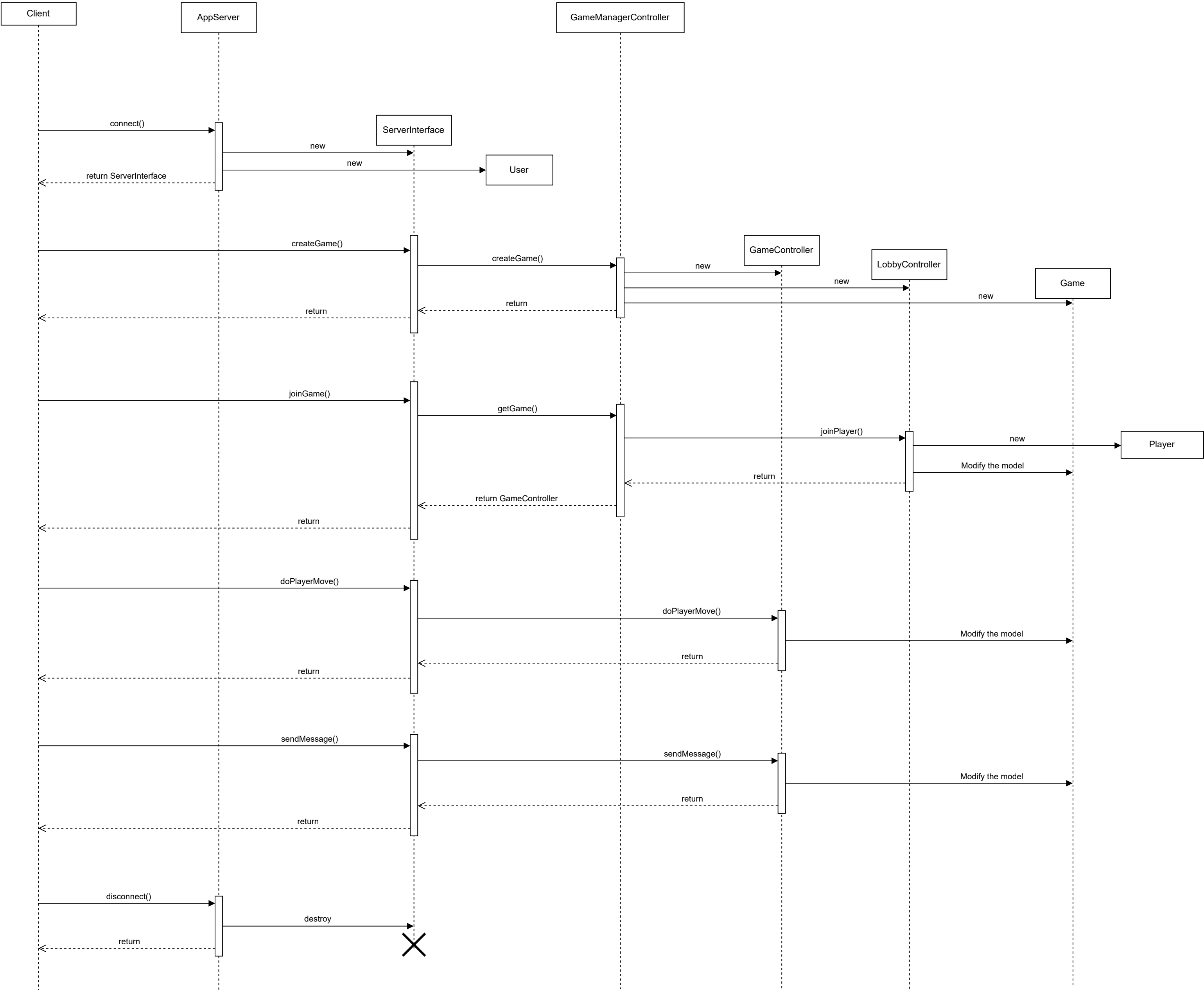
Client to Server interaction sequence
