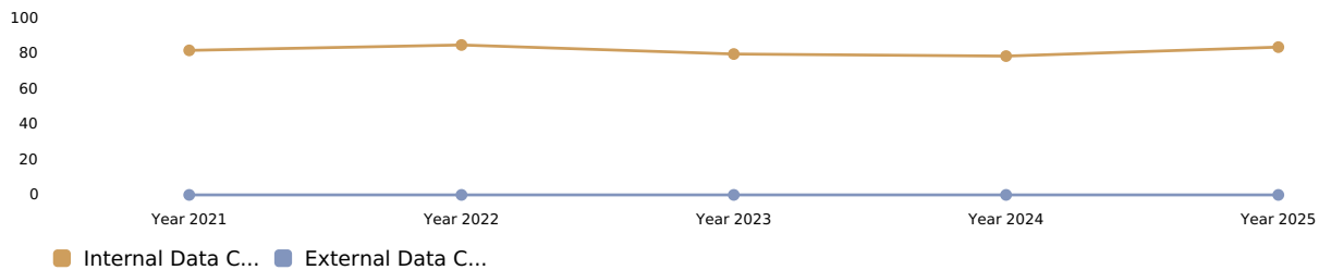
Internal vs External Data Comparison
