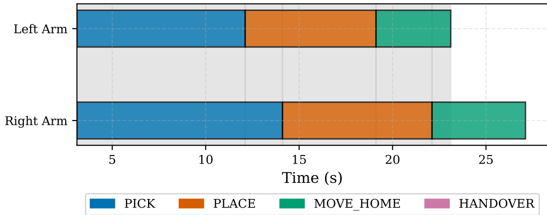
Bimanual Timeline (B-EXP1)
