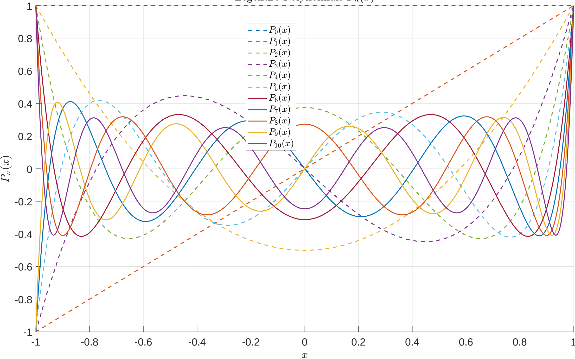
Legendre Polynomials P_n(x)
