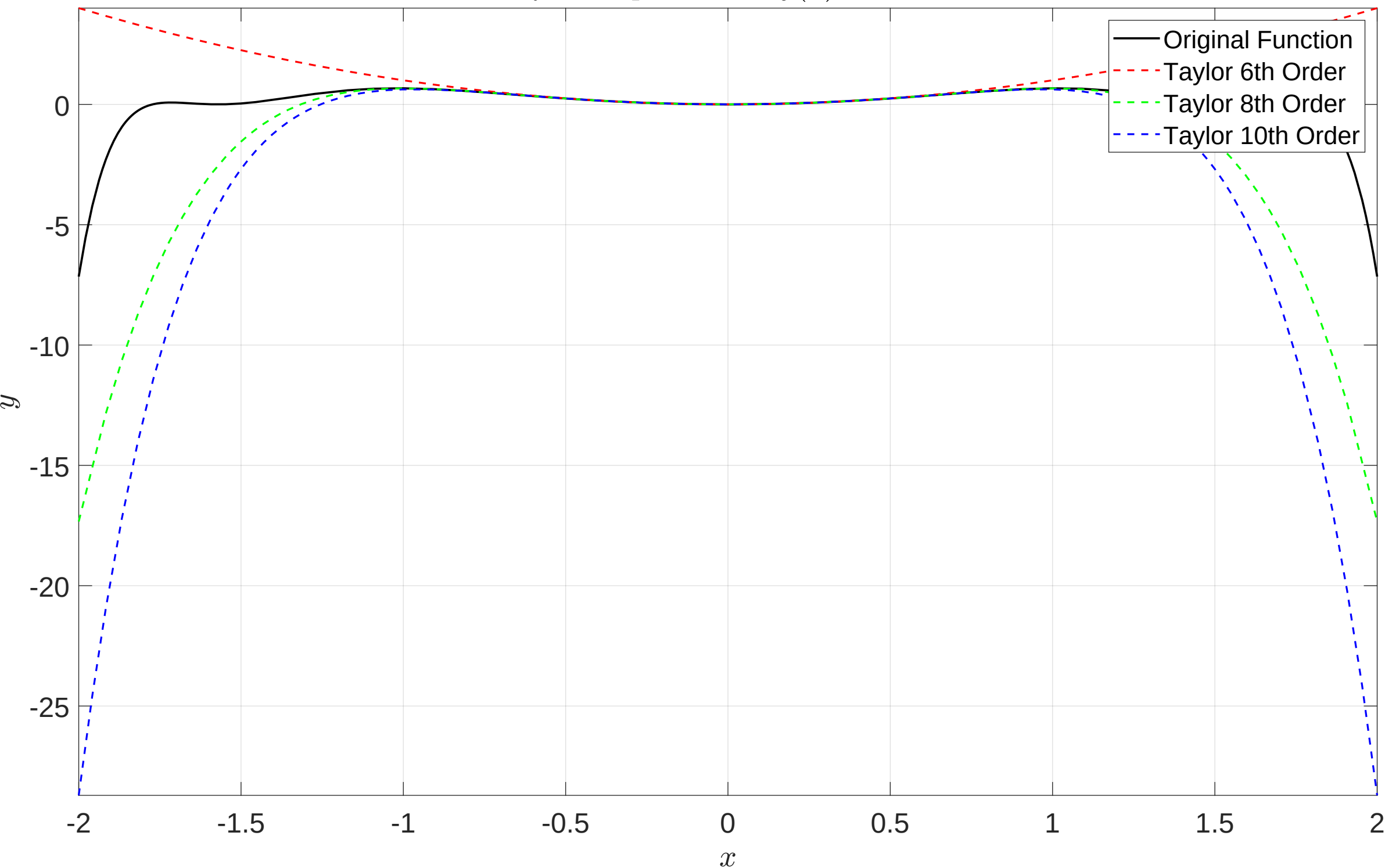
Taylor Expansion of y(x) at x = 0
