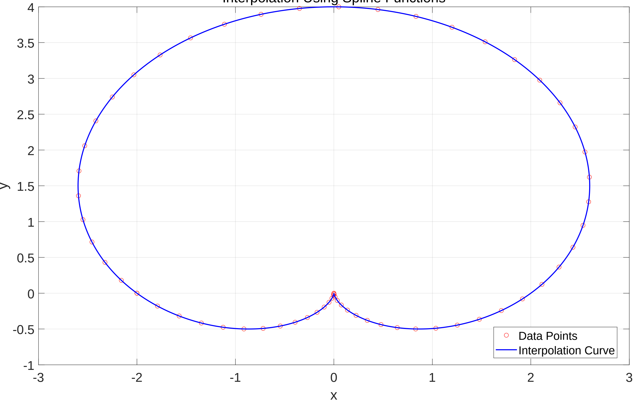
Interpolation Using Spline Functions
