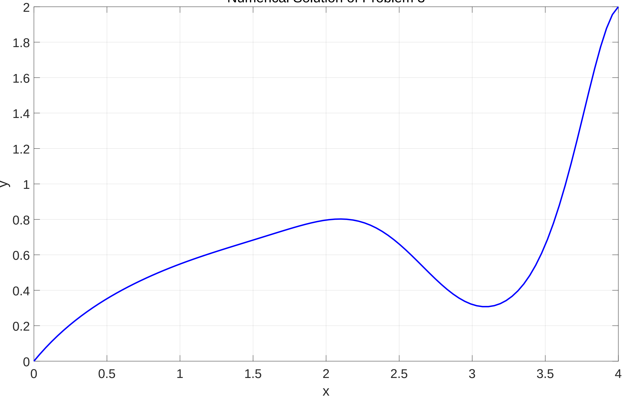
Numerical Solution of Problem 3
