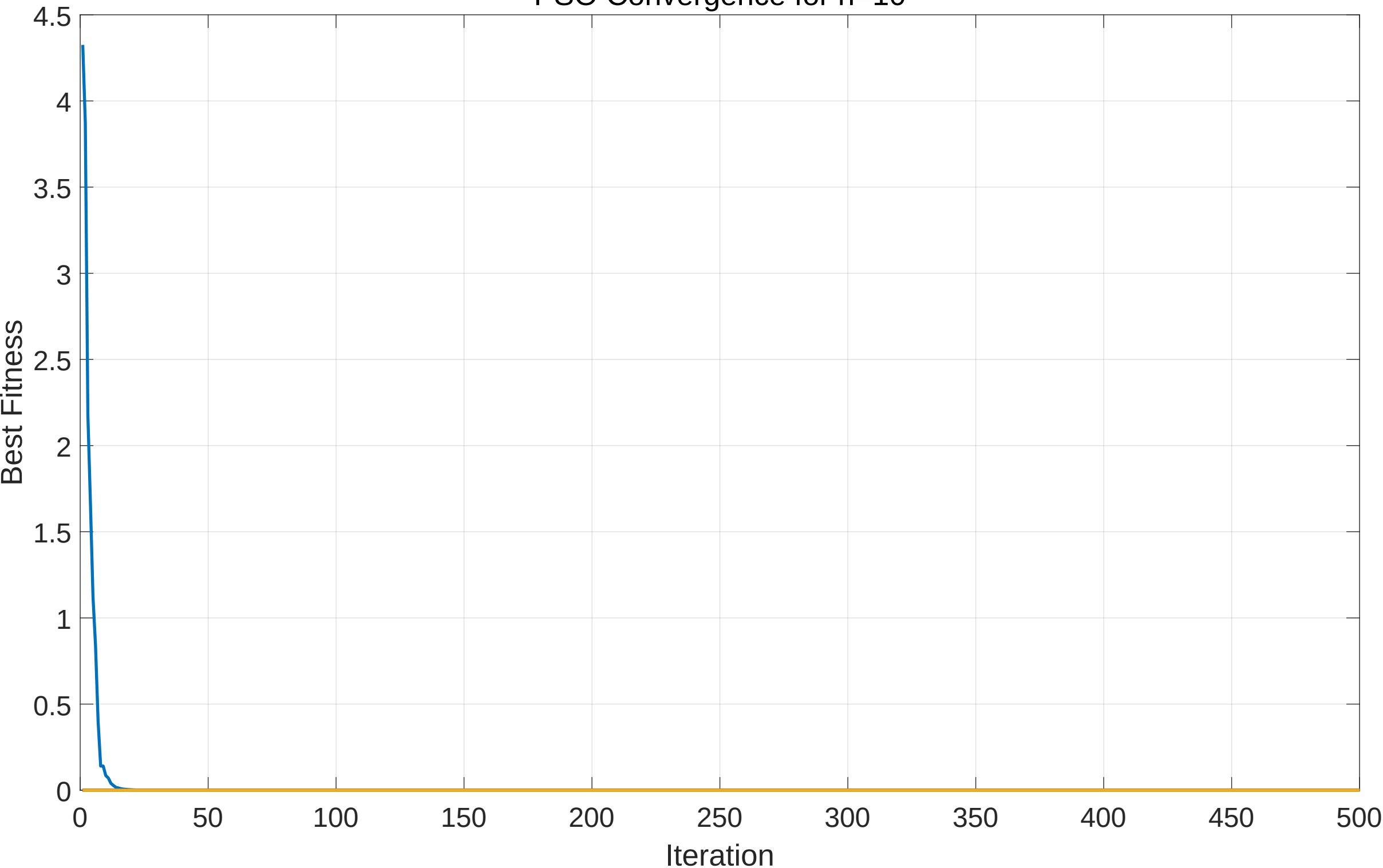
PSO Convergence for n=10
