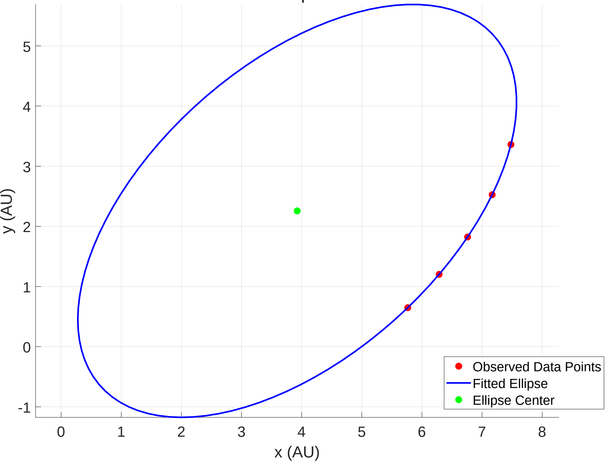
Asteroid Elliptical Orbit
