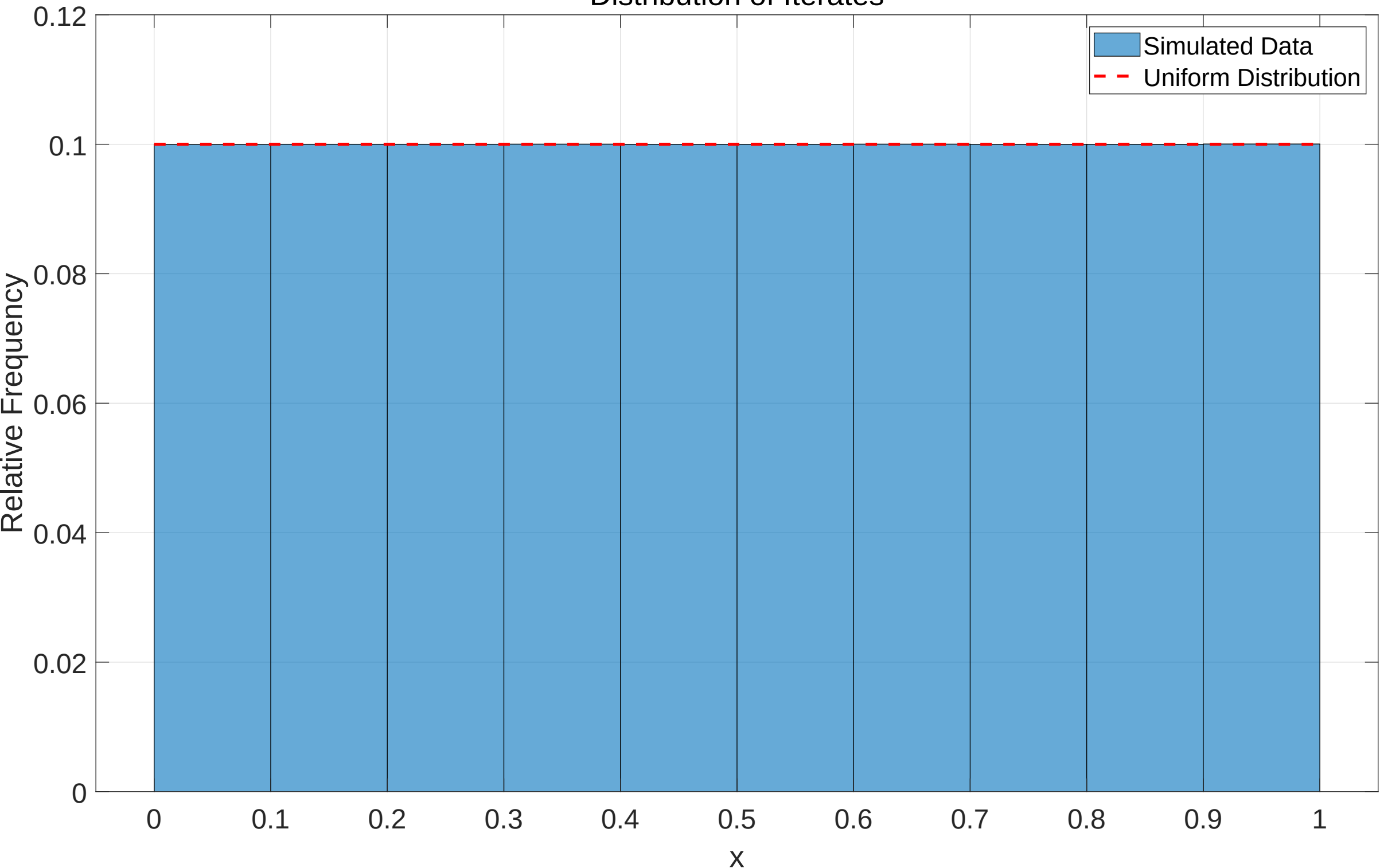
Distribution of Iterates
