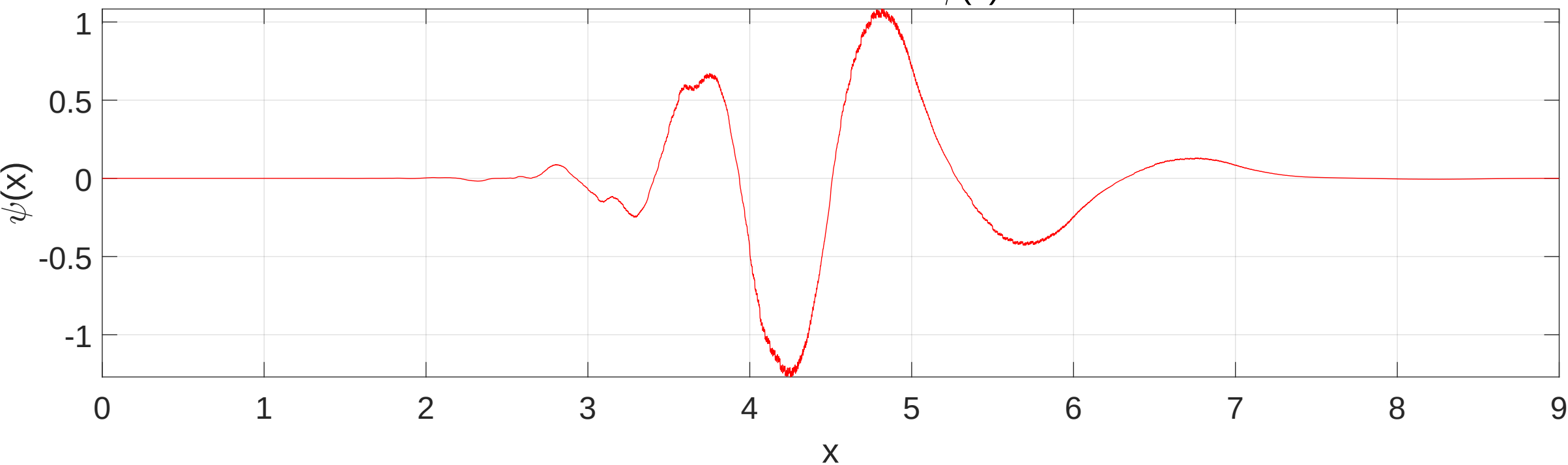
Wavelet Function \psi(x)
