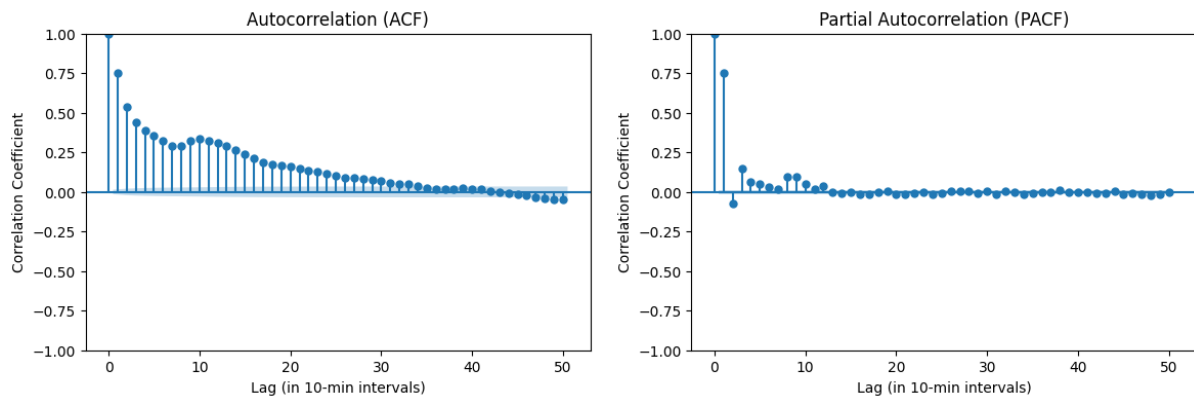
Figure 7: ACF/PACF plots of the target variable, Appliances
