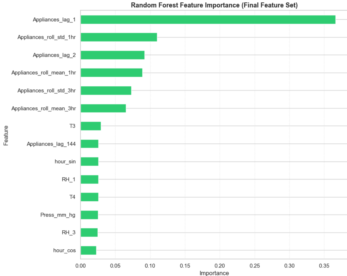
Figure 10: Random Forest feature importance
