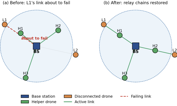
Fig. 1. Self-healing scenario. (a) Initial layout: helper drones (H1–H3) are inside coverage; L1 holds a direct link to the base that is about to fail (red dashed), while L2 is already isolated. (b) After the spring-damper repositioning, helpers move outward to bridge each disconnected drone with the base via a multi-hop relay.
