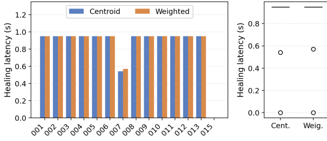
Fig. 2. Healing-latency distribution across the 15 scenarios. Left: per-scenario values for both controllers. Right: aggregate boxplot.
