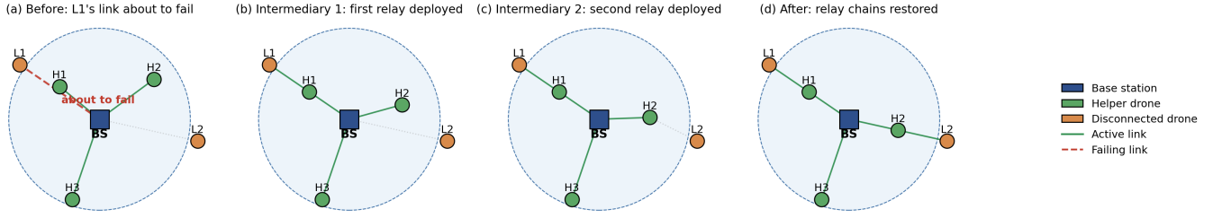
Fig. 1. Self-healing scenario. (a) Initial layout: helper drones (H1–H3) are inside coverage; L1 holds a direct link to the base that is about to fail (red dashed), while L2 is already isolated. (b) After the spring-damper repositioning, helpers move outward to bridge each disconnected drone with the base via a multi-hop relay.
